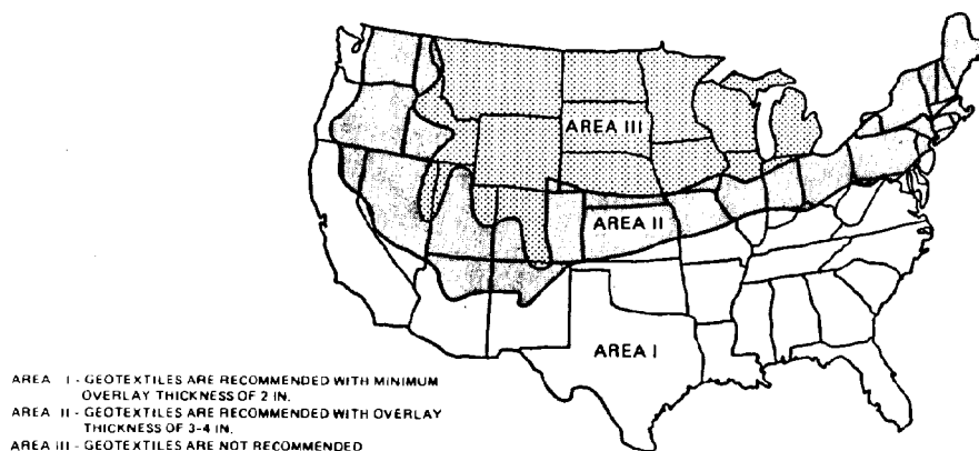
Figure 14-2. Location Guide for the Use of Geotextiles in Retarding Reflective Cracking.
