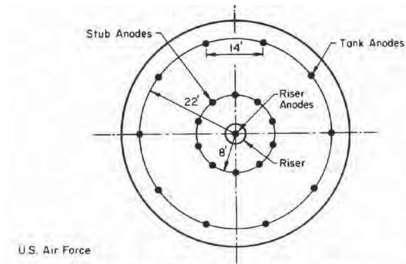
Figure D-8. Anode spacing for elevated steel water tank.
