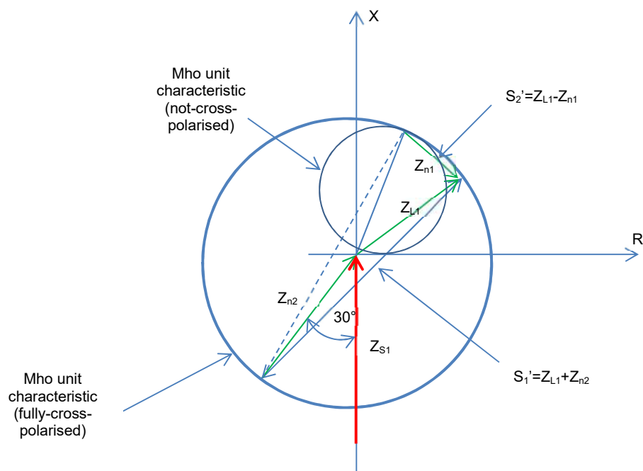
Figure 13. Diagram of enhancing protection relay resistive coverage for fully cross-polarised characteristic
