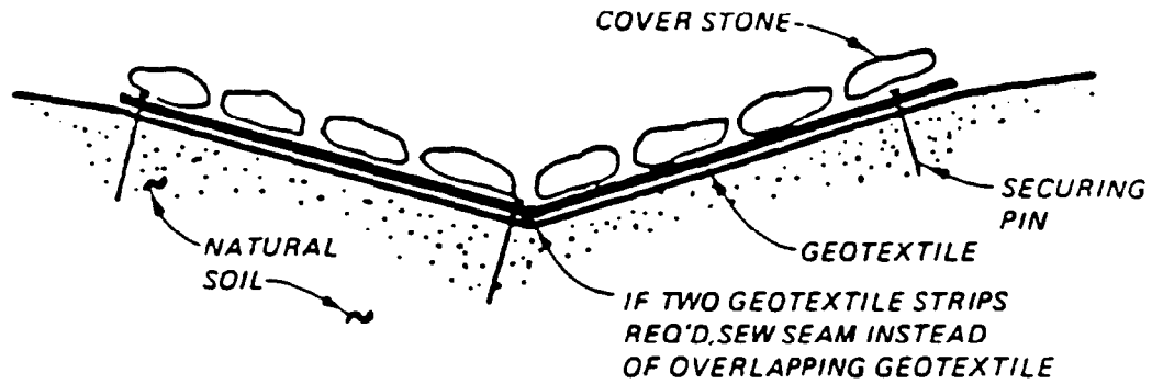
CROSS SECTION OF GEOTEXTILE-LINED DITCH
