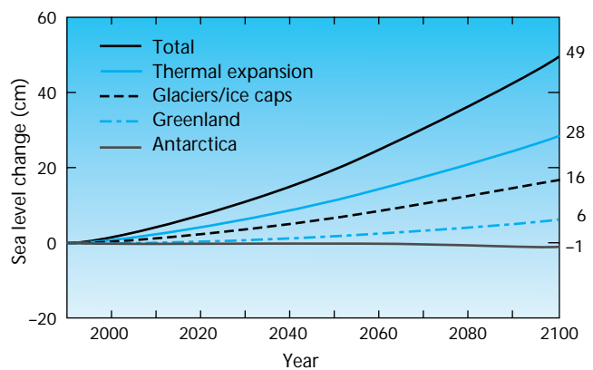
Figure 13. The individual contributions to the “MID” sea level rise case shown in Figure 11 (reproduced from SAR WGI, Figure 7.8).
