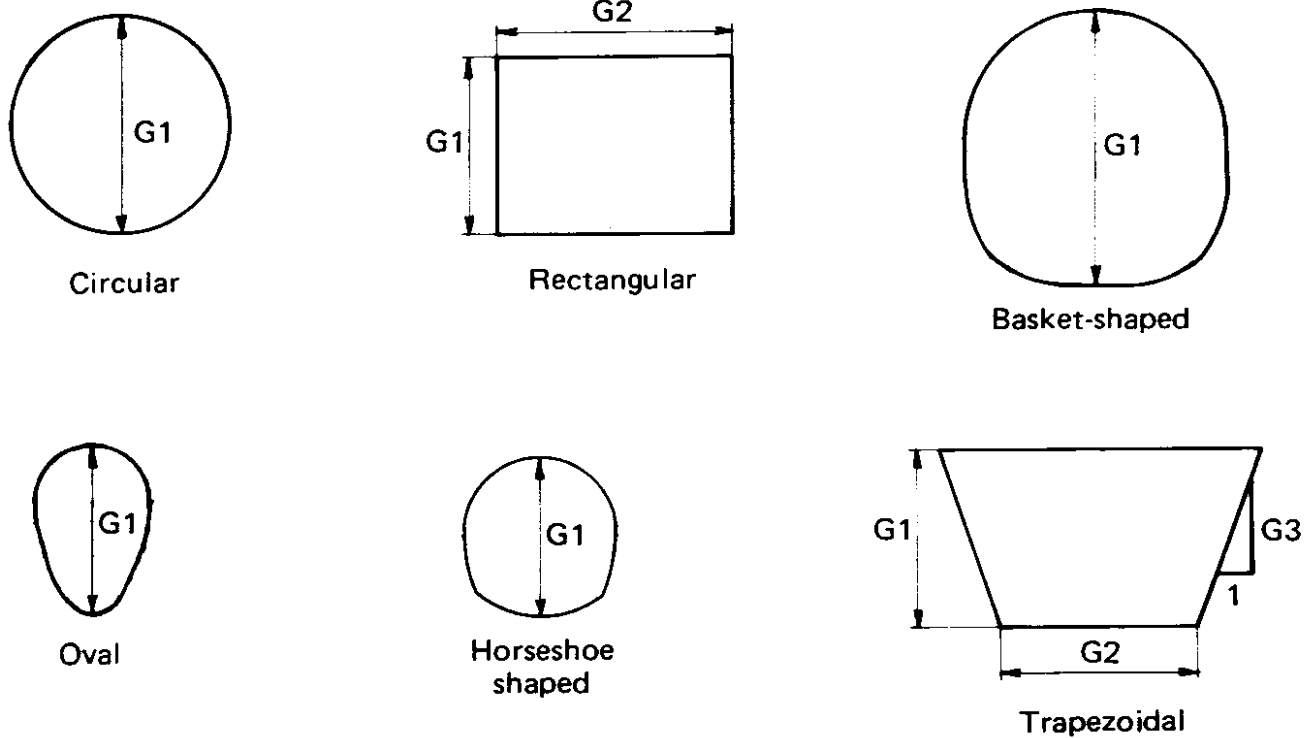
Figure A-4 Standard pipe sections provided in EXTRAN Block.
