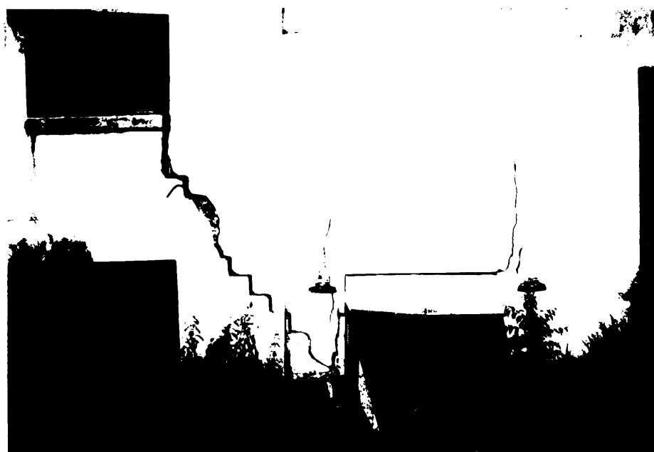
b. Diagonal and vertical cracks
