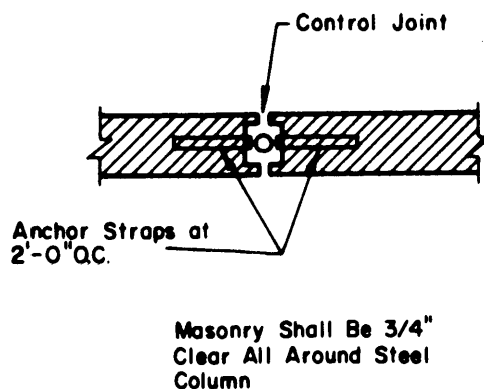
STEEL COLUMN IN INTERIOR WALL
