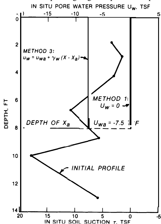
Figure 5-2. Example application of equilibrium pore water pressure profile for a site near Hayes, Kansas.
