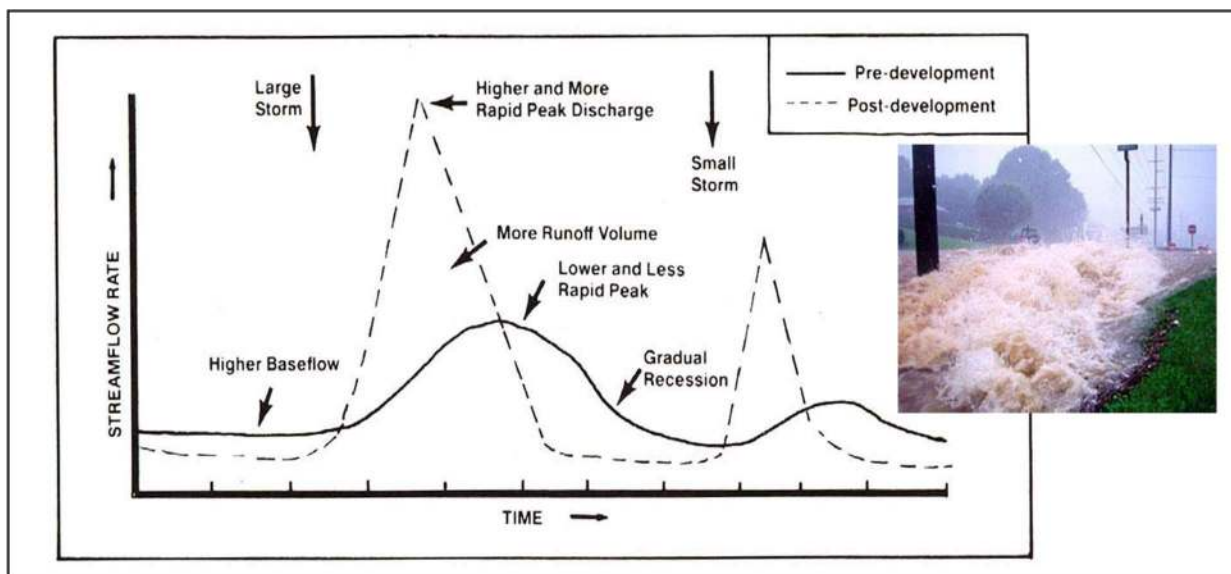
Figure 13: Comparison of Urban and Rural Hydrographs
