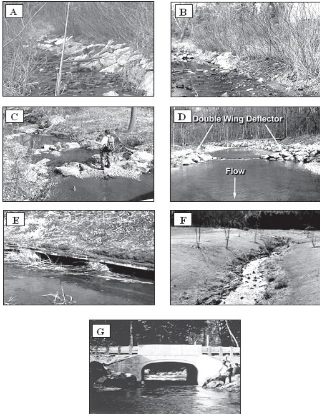
Figure 20: The Seven Basic Types of Stream Repair Techniques
