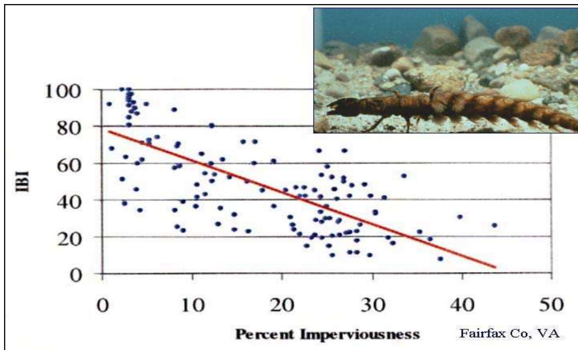
Figure 17: Relationship Between Subwatershed IC and Aquatic Insect Diversity
