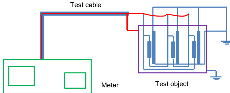
Figure 5. Power transformer RVM test setup
