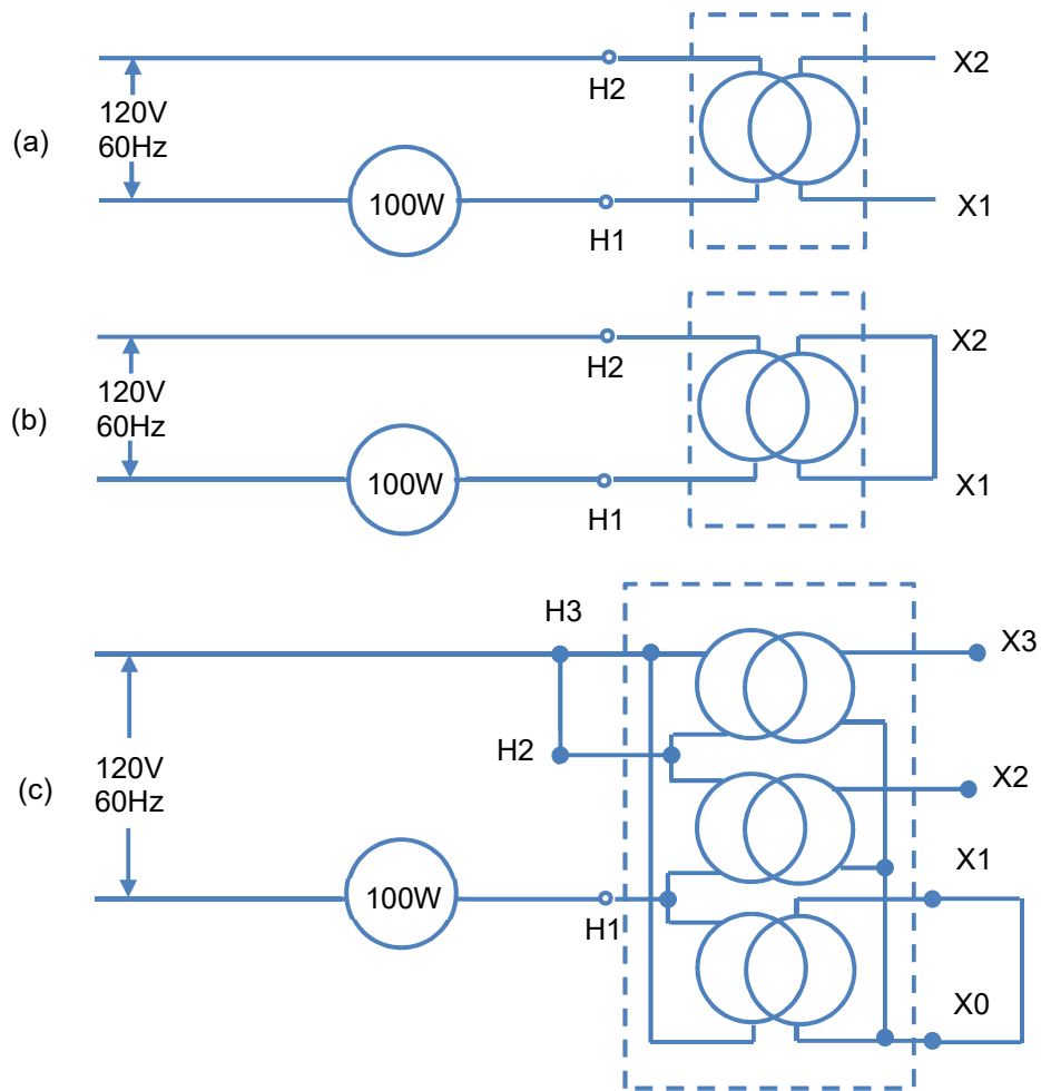
Figure 2. Transformer winding continuity verification
