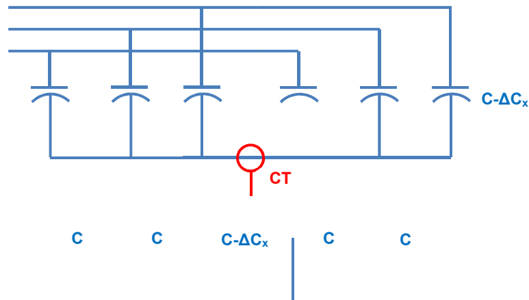
Figure 7. Compensating faults in the same phase lead to no unbalance signal
