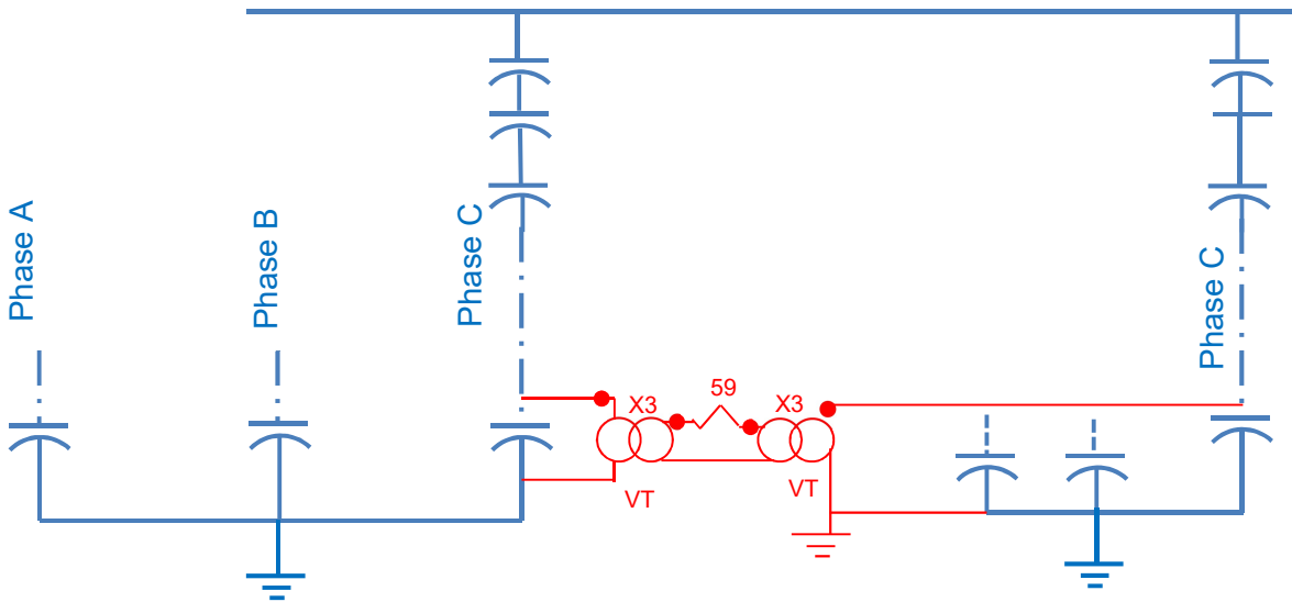
Figure 16. Voltage differential arrangement for grounded double wye shunt capacitor bank
