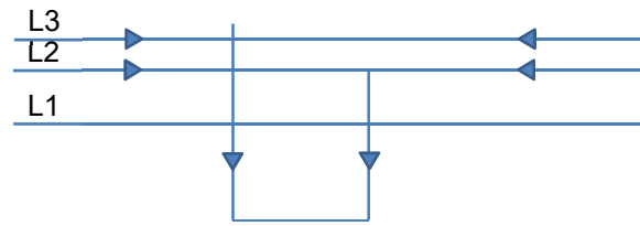
Line to Line Fault
