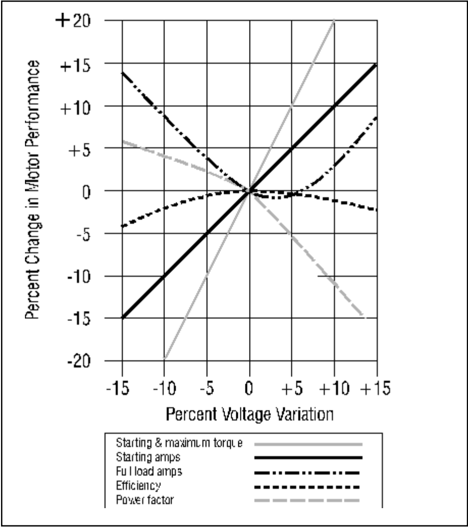
Figure 9-1 Effect of Voltage Variation on Induction Motor Performance Characteristics
