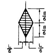
DISTRIBUTION OF BEARING PRESSURES BENEATH RECTANGULAR FOOTINGS
