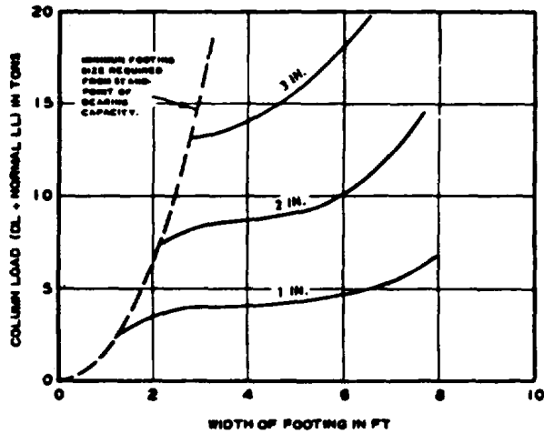
EXAMPLE OF CHARTS FOR SELECTING ALLOWABLE BEARING PRESSURES AND FOOTING SIZES RESULTING IN EQUAL SETTLEMENT OF FOOTINGS. CURVES BASED ON EQ 1.
