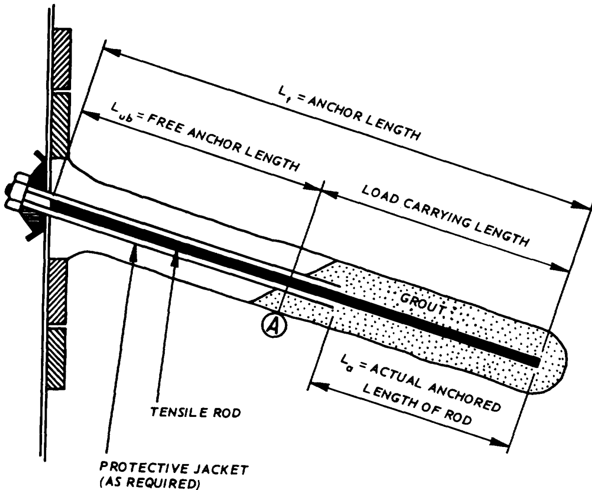
Figure 14-13. Typical tieback details.
