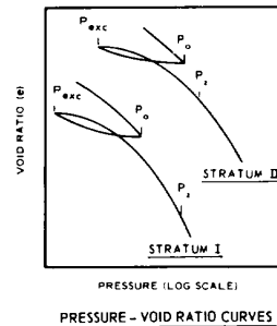
Figure 5-4. Example of settlement analysis.
