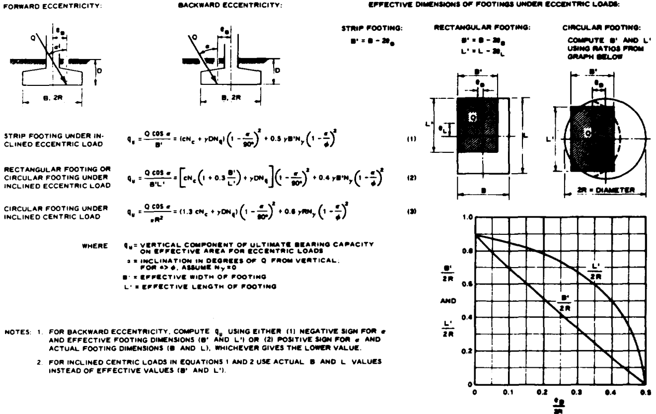
Figure 6-3. Ultimate bearing capacity of shallow foundations under eccentric inclined loads.
