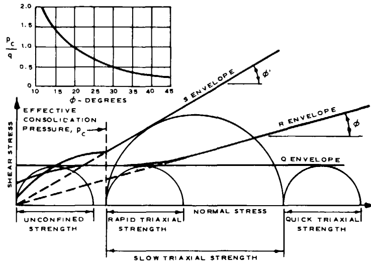
b. TYPICAL FAILURE ENVELOPES FOR Q, R, AND S TESTS
