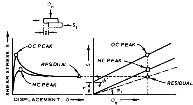
d. SHEARING RESISTANCE OF OVER-CONSOLIDATED (OC) AND NORMALLY-CONSOLIDATED (NC) CLAYS
