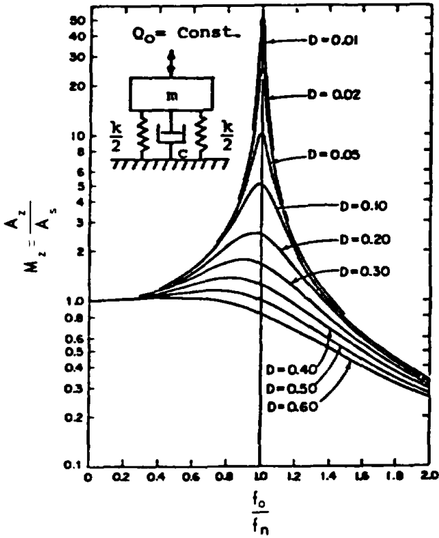
(a) CONST. FORCE AMPLITUDE EXCITATION Q = Q_0 \sin \omega t
