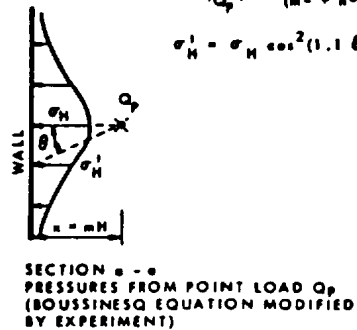
Figure 14-5. Horizontal pressures on walls due to surcharge.
