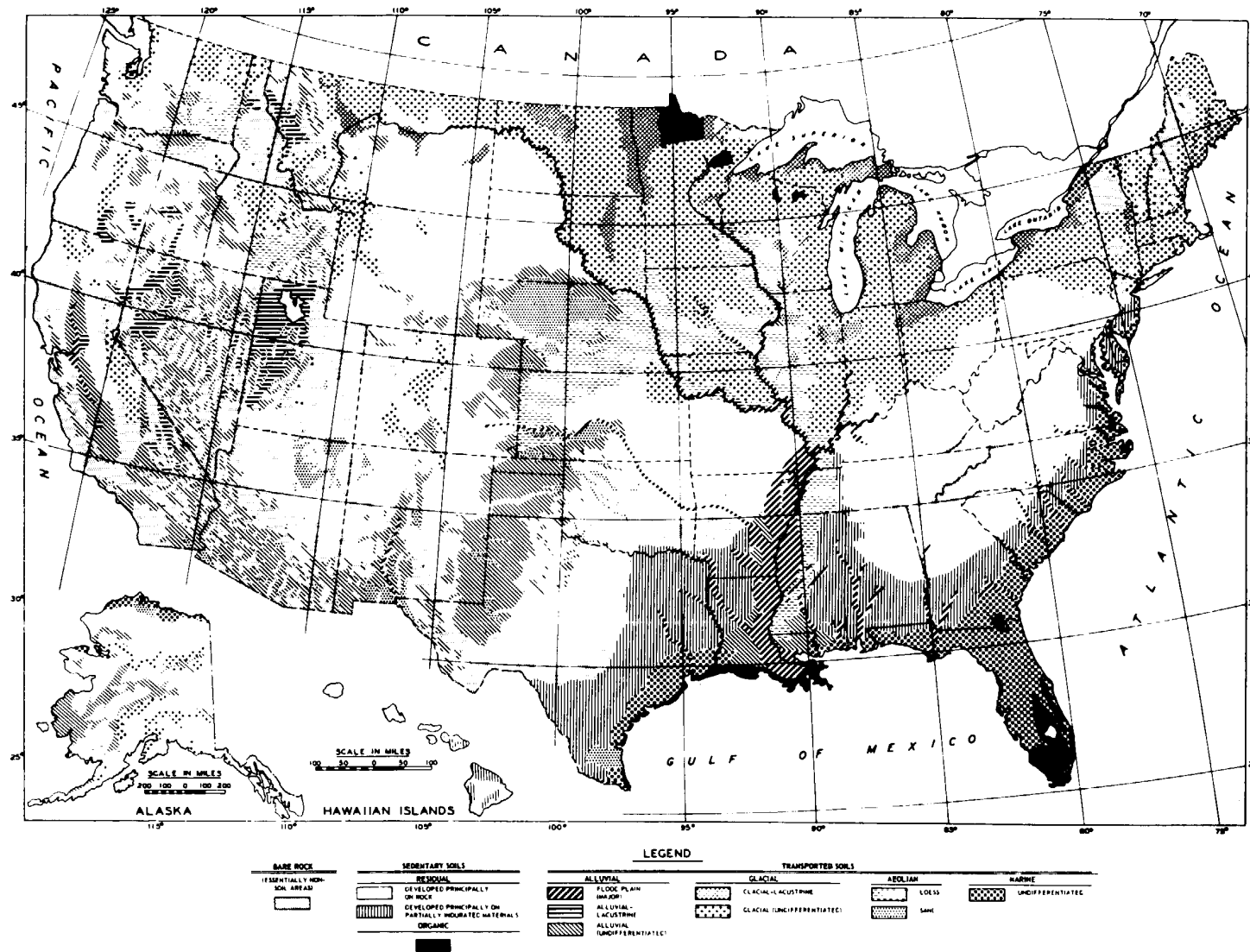
Figure 2-1. Distribution of natural soil deposits in the United States.
