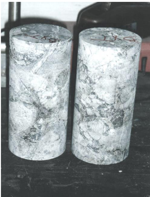
Fig. 20. 100 mm diameter by 200 mm long specimens of Braden Breccia from the El Teniente mine in Chile
