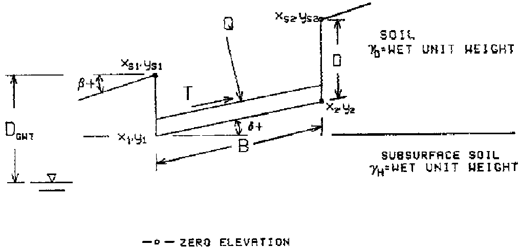
Figure 4-7. Shallow foundation with slope and base tilt
