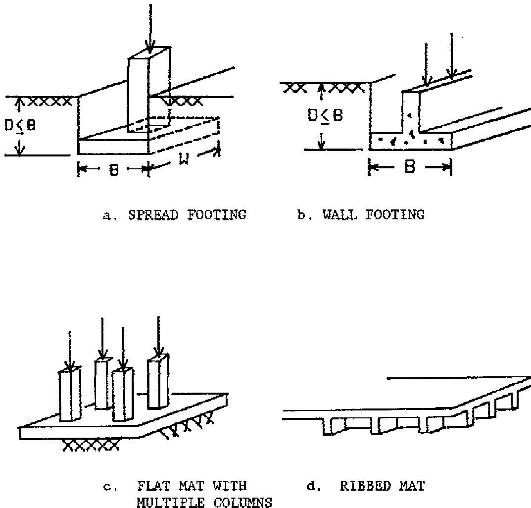
Figure 1-1. Shallow Foundations
