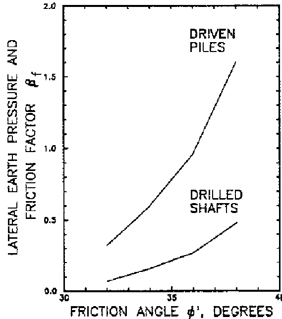
Figure 5-5. Lateral earth pressure and friction angle factor \beta as a function of friction angle prior to installation (Data from Meyerhof 1976 and Poulos and Davis 1980)
