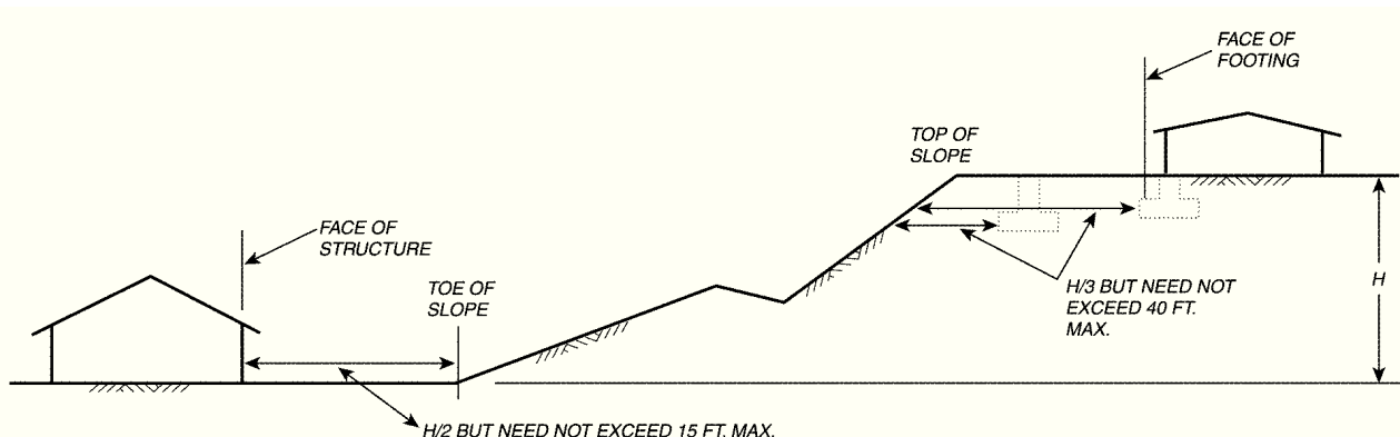
FIGURE 1805.3.1 FOUNDATION CLEARANCES FROM SLOPES
