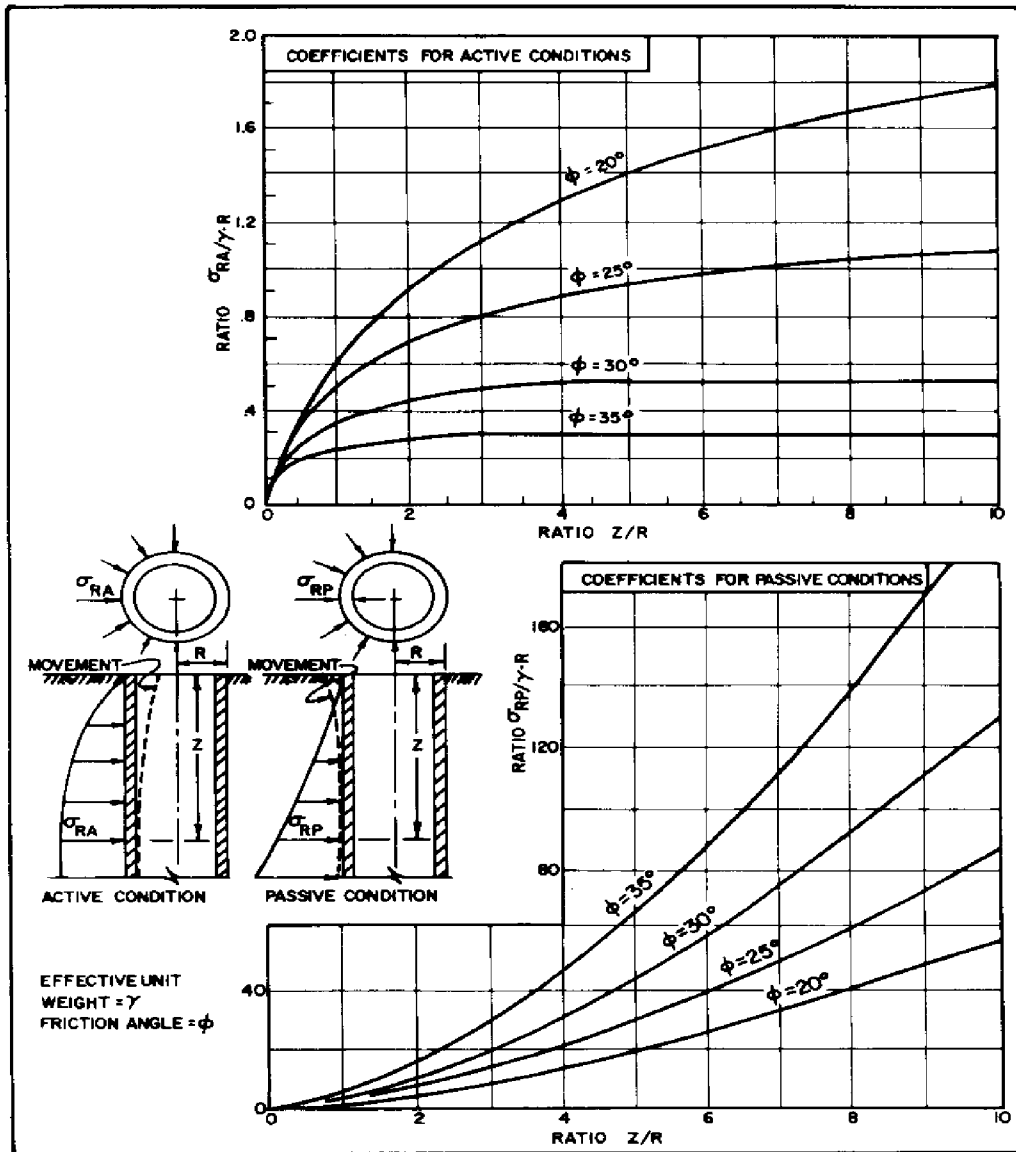
FIGURE 24 Coefficients for Active or Passive Pressures on Underground Cylindrical Shafts or Silos
