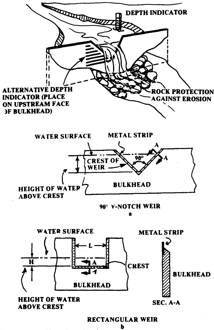
Figure 6.7 - Standard Weirs
