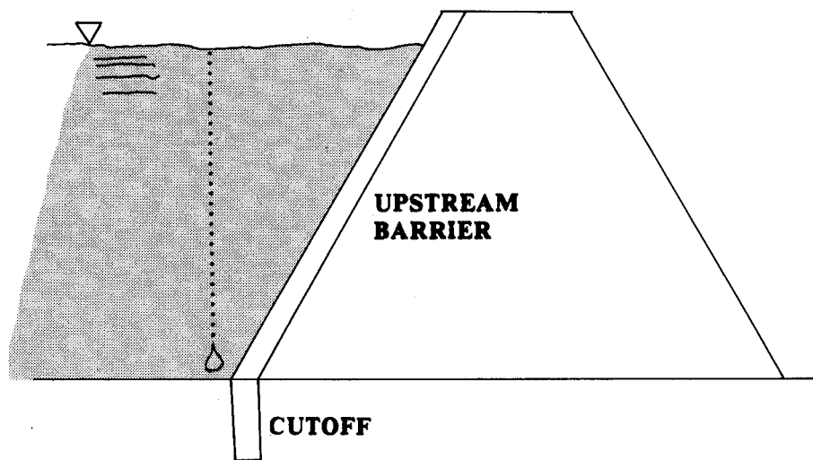
Figure 2.2 Embankment Dam
