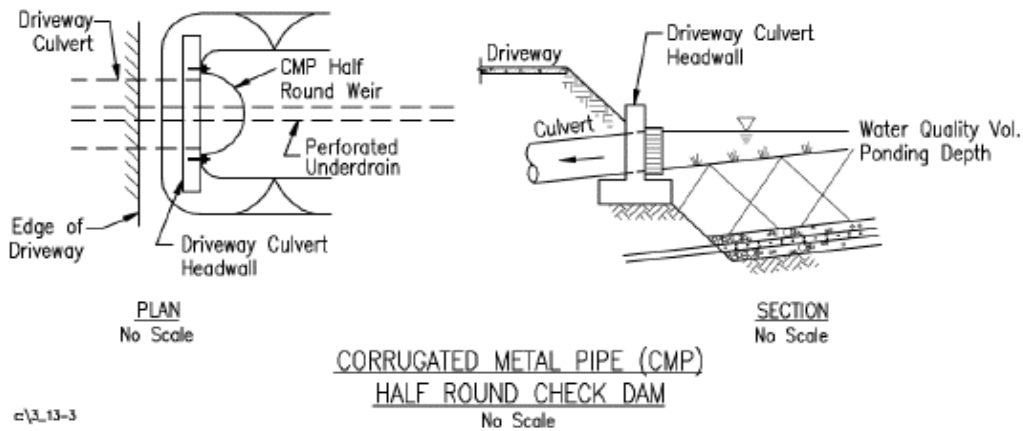
Figure 6-8 Typical Check Dam Configurations (VA DEC, 1999)
