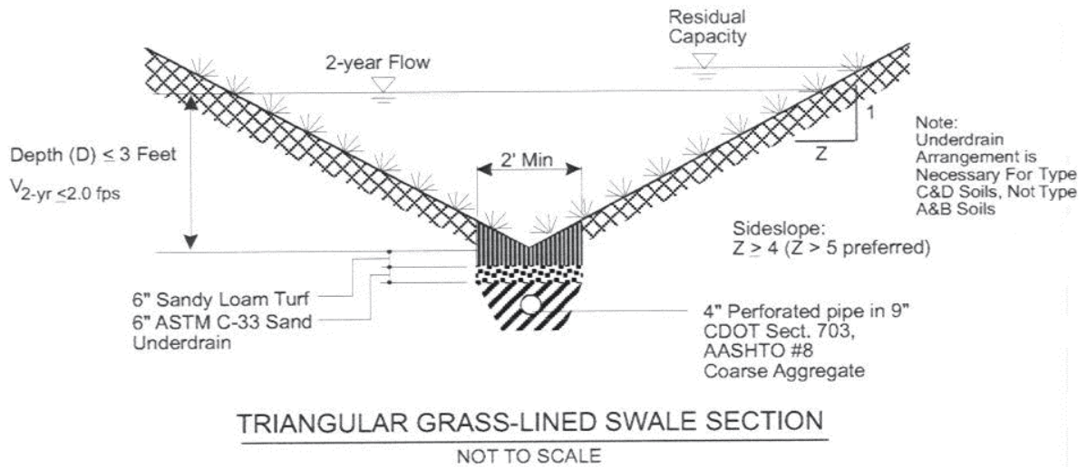
Figure 6-5 Grass Swale Profile and Section (UDFCD, 1999)
