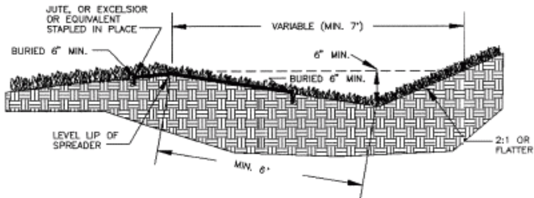
LEVEL SPREADER WITH VEGETATED LIP
