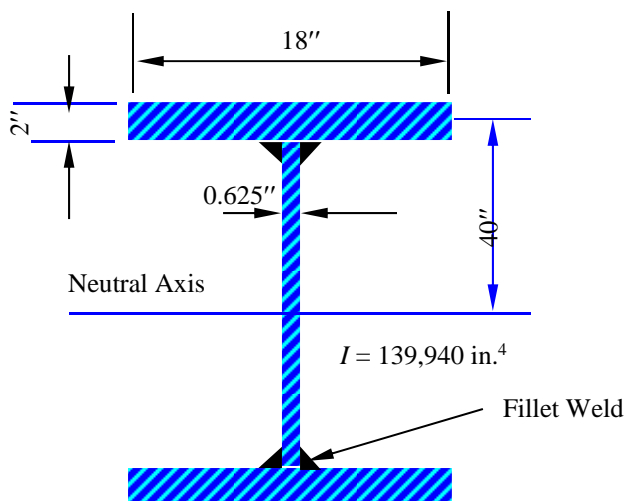
Figure 9.7-9 Flange-to-Web Welds
