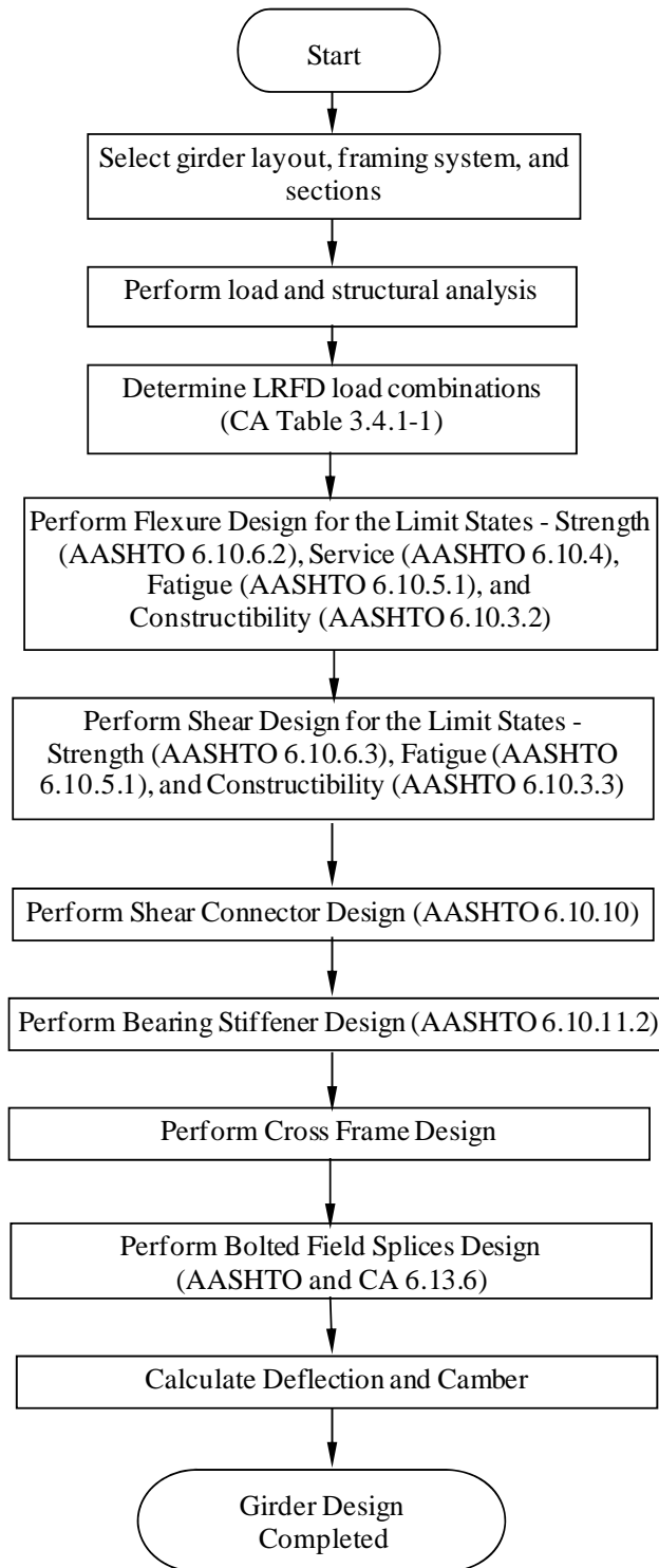
Figure 9.6-1 Steel I-Girder Design Flowchart
